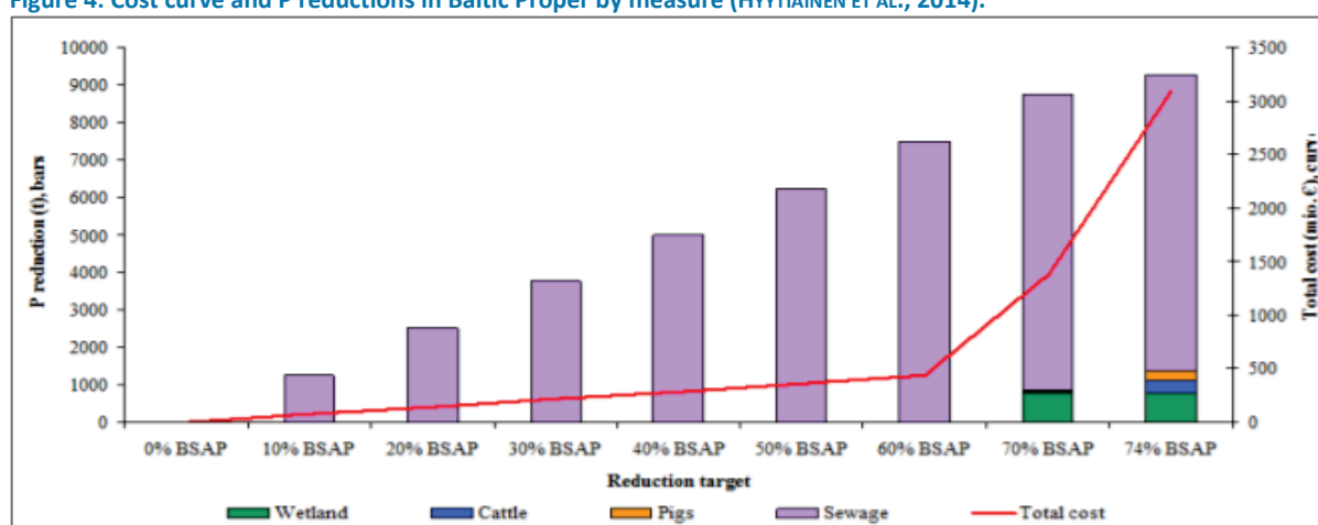
Figure 4: Cost curve and P reductions in Baltic Proper by measure (HYTTIÄINEN ET AL., 2014).
