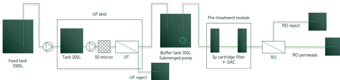
Figure 11: Process flow of test installation.
