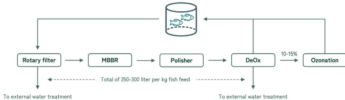
Figure 8: The internal water treatment process
